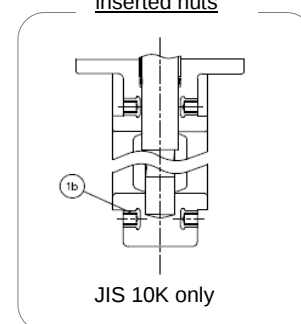
Detail of inserted nuts
