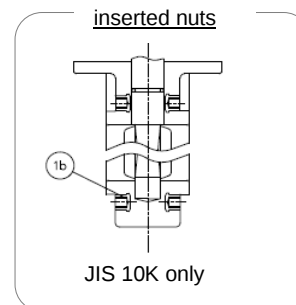
Detail of inserted nuts
